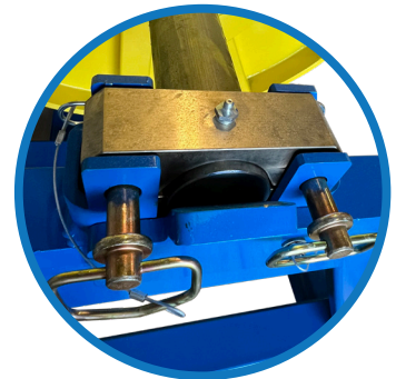
SAFETY SHAFT LATCHES
