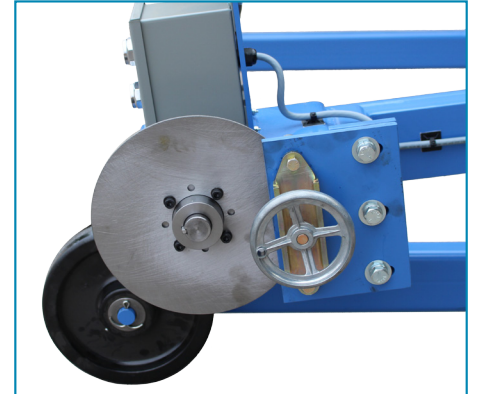
10" Mechanical Brake
