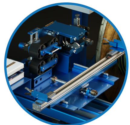
CABLE TRANSPORT & CUTTING SYSTEM
