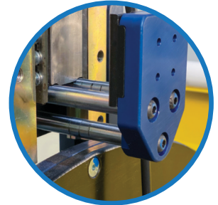
INTEGRATED GRIPPER CUTTER
